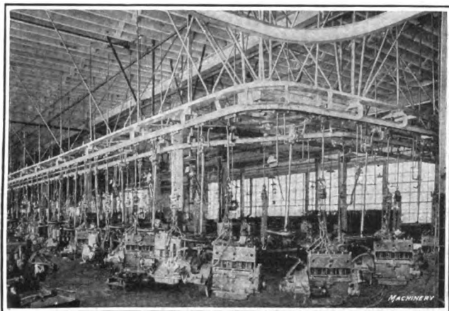
Fig. 22—In large plants, such as that of the Willys-Overland Co., a visitor is bound to be impressed by the variety of equipments employed for handling raw materials and product. For instance, the preceding illustration shows an apron-type conveyor for carrying assembled motors, and in this view the same class of work is being done by a trolley system installed by the Link-Belt Co.
